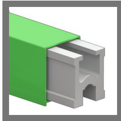
Bolt Jointed Aluminum Busbar System
