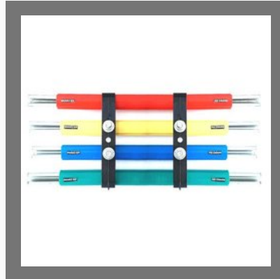
DSL Busbar System 60Amp Galvanized Iron
